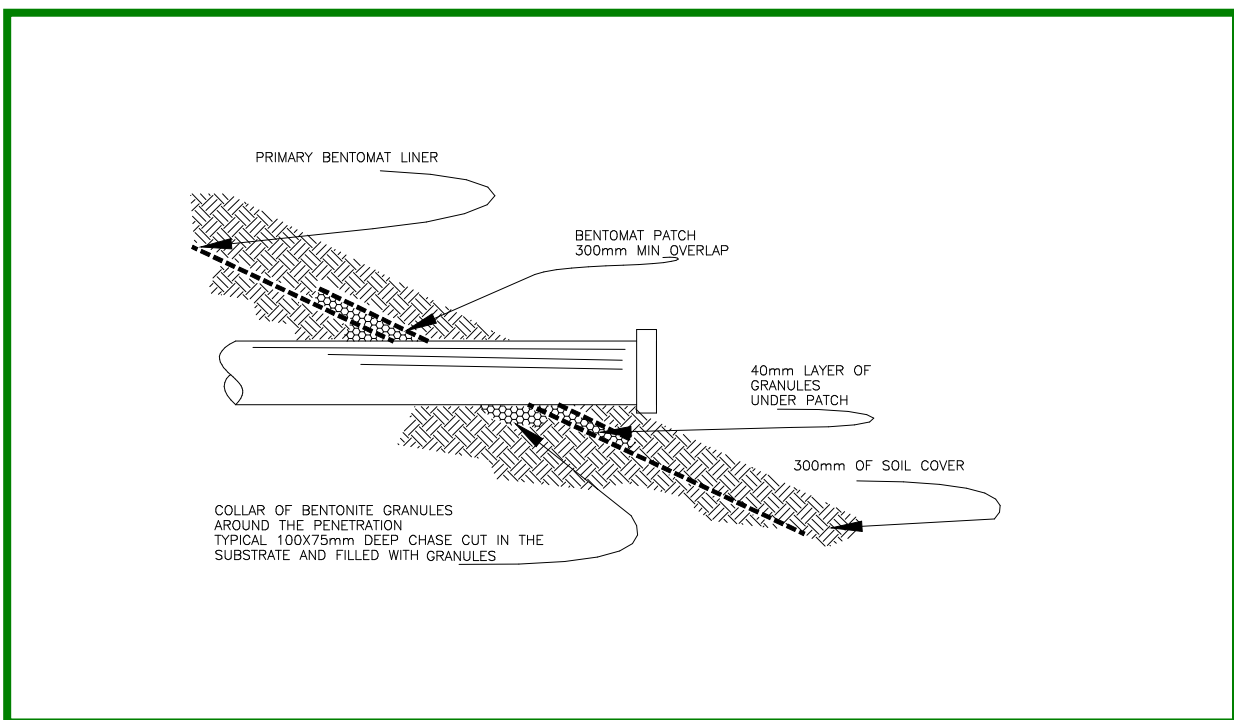
Figure 4a. Cross-section of a horizontal pipe penetration.
