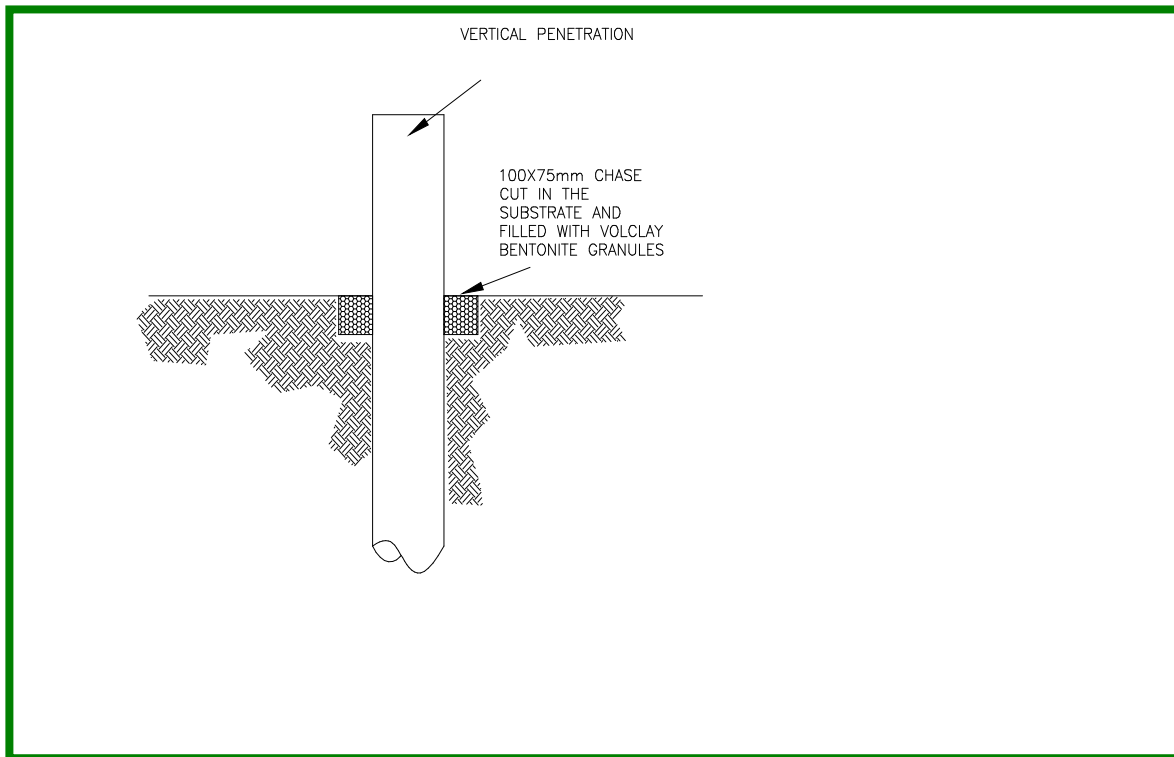
Figure 5a. Cross-section of a vertical penetration.
