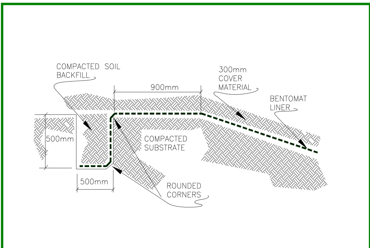
Figure 2. Typical anchor trench location and dimensions.
