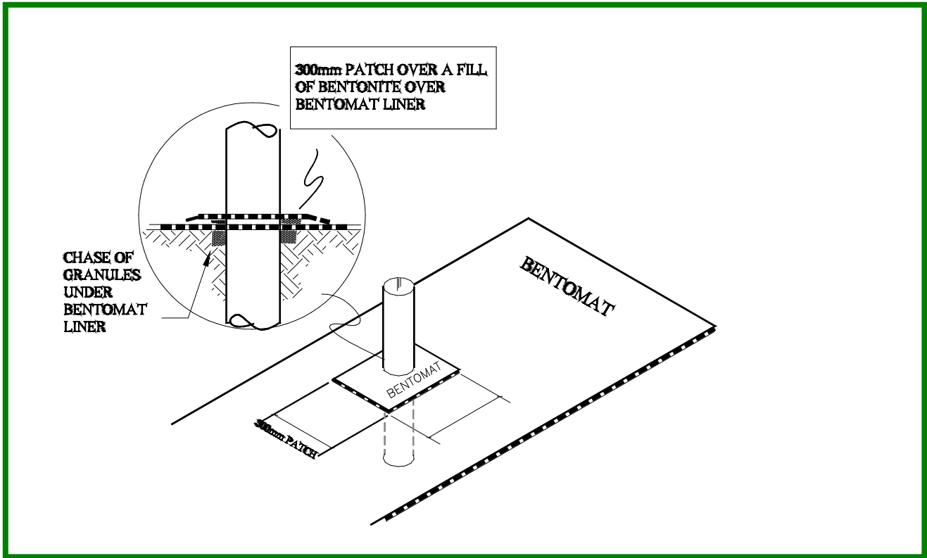
Figure 5b. Isometric view of completed vertical penetration.
