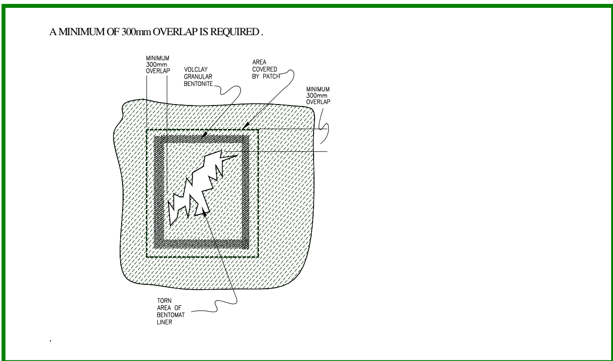
Figure 7. Damage repair by patching.
