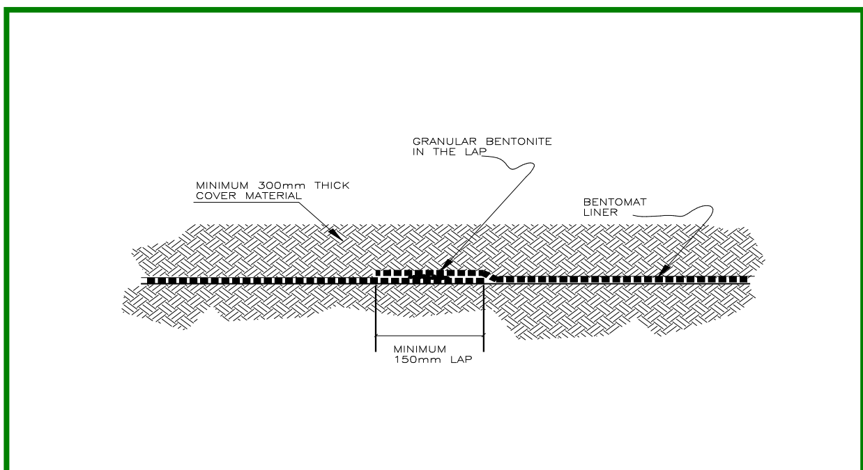
Figure 3. Bentonite-enhanced overlapped seam.
